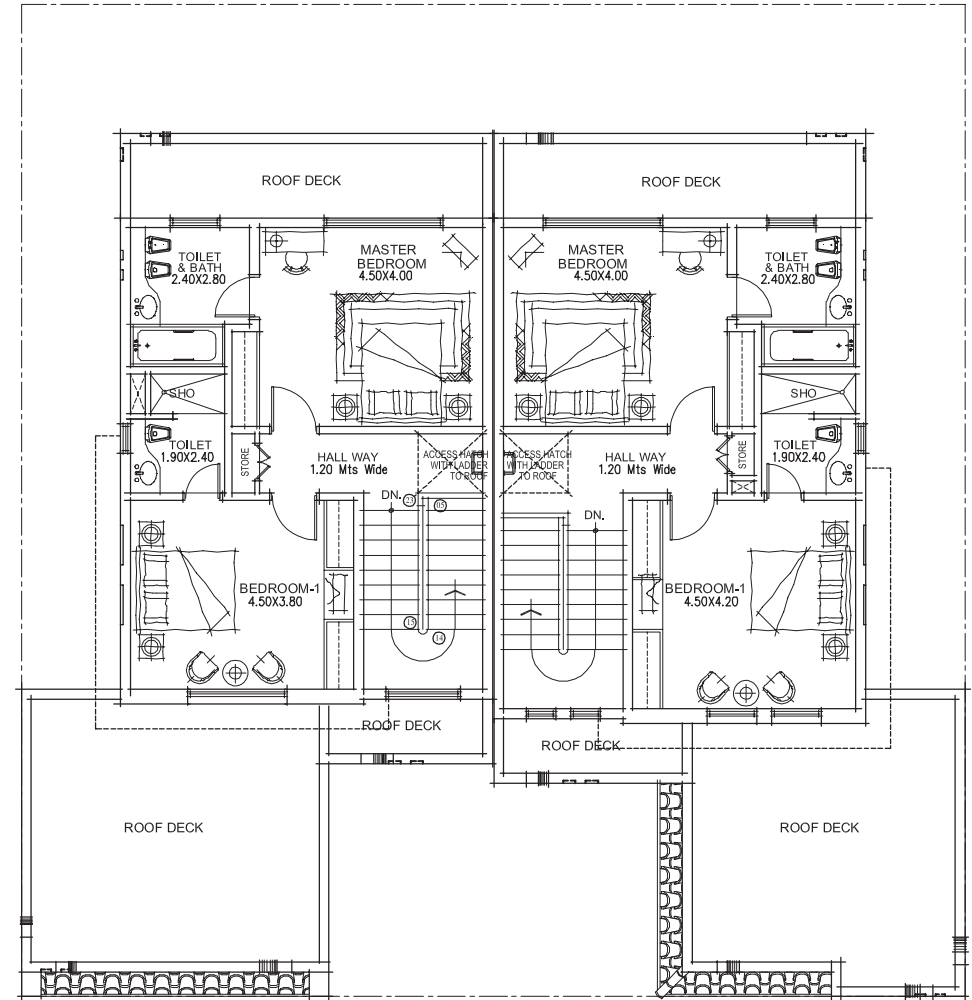
First Floor
